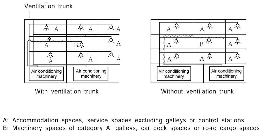
Fig 8.7.5 Examples for arrangements of Ventilation system
